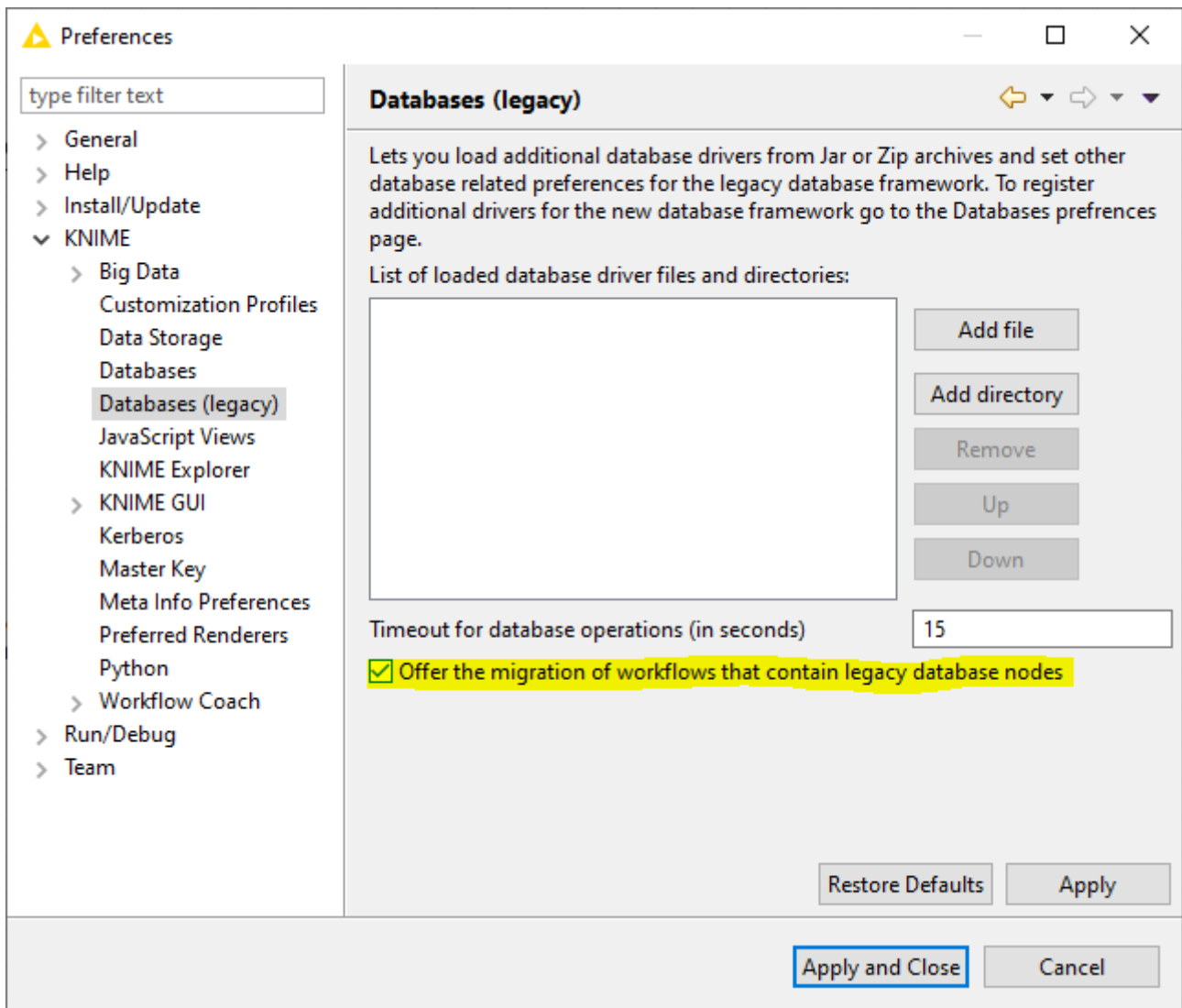
Figure 52. Disabling migration message
