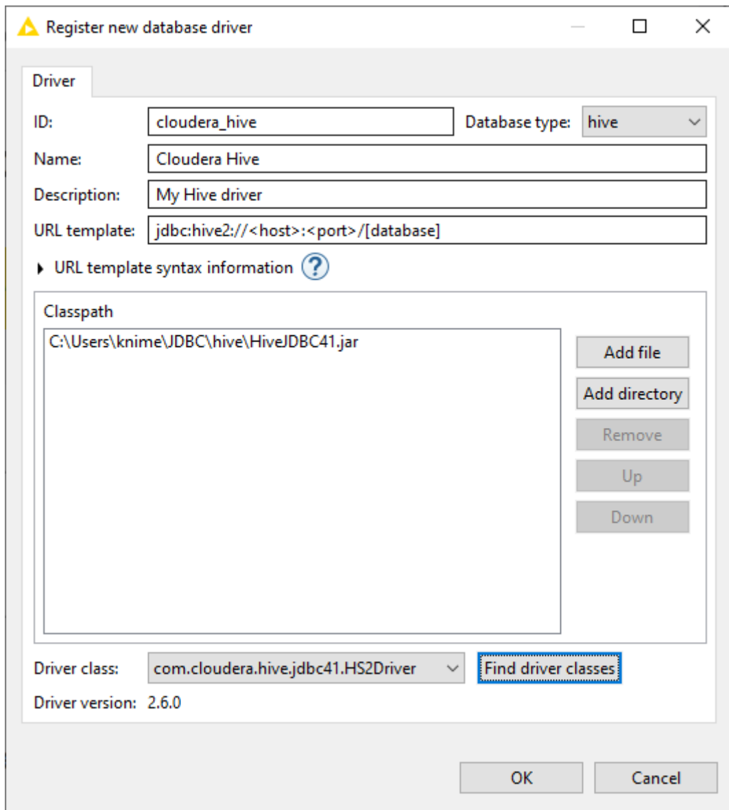
Figure 21. Register new Apache Hive driver
