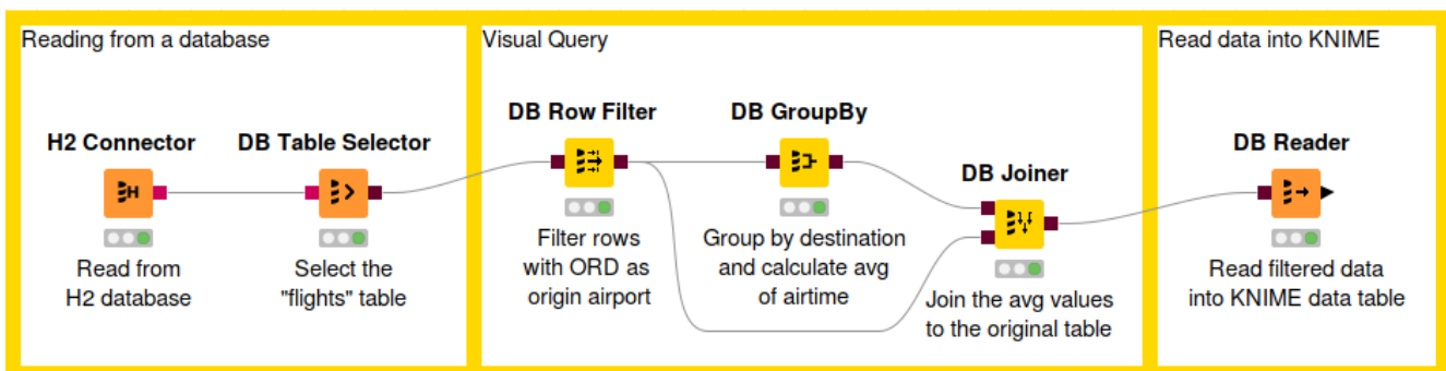
Figure 29. Example of a workflow that performs in-database data manipulation
