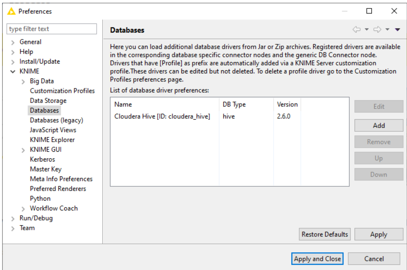
Figure 22. Database Preference page
