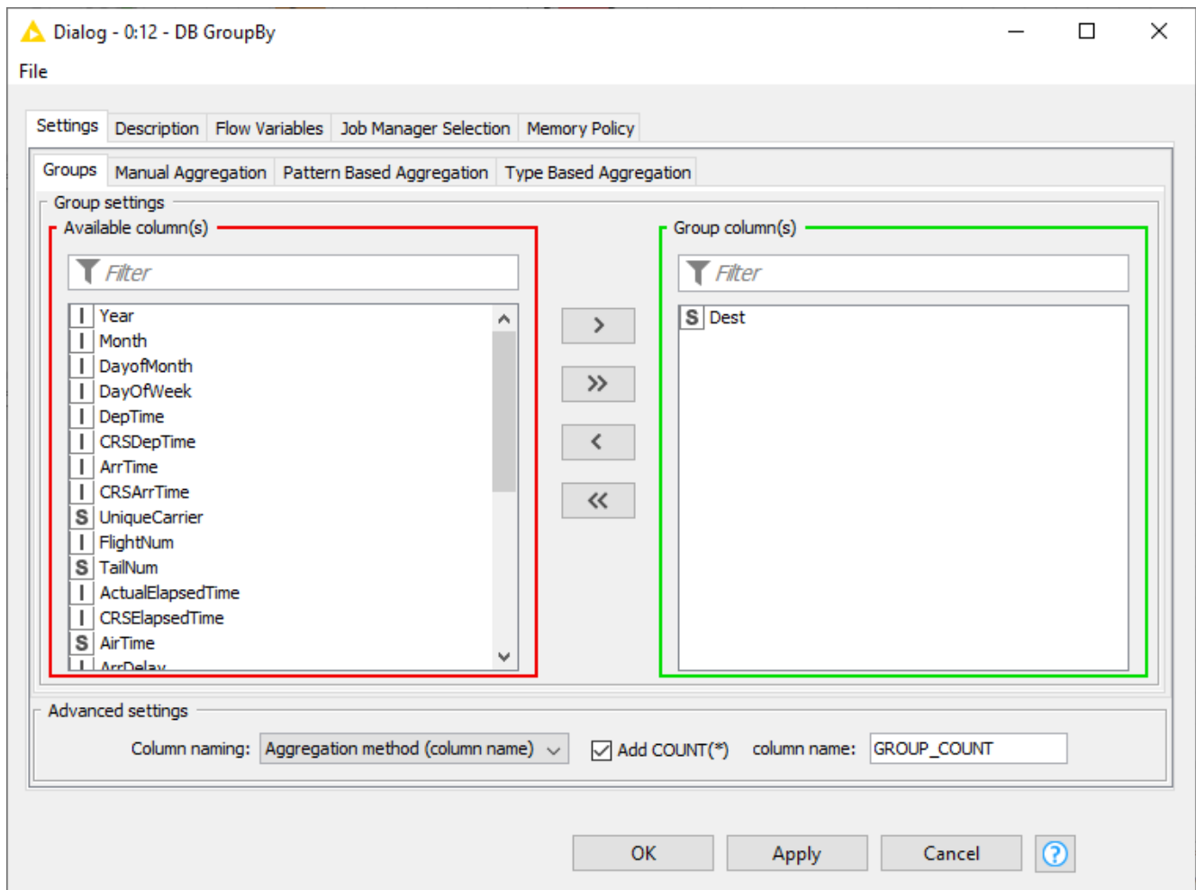
Figure 32. DB GroupBy: Group Settings
