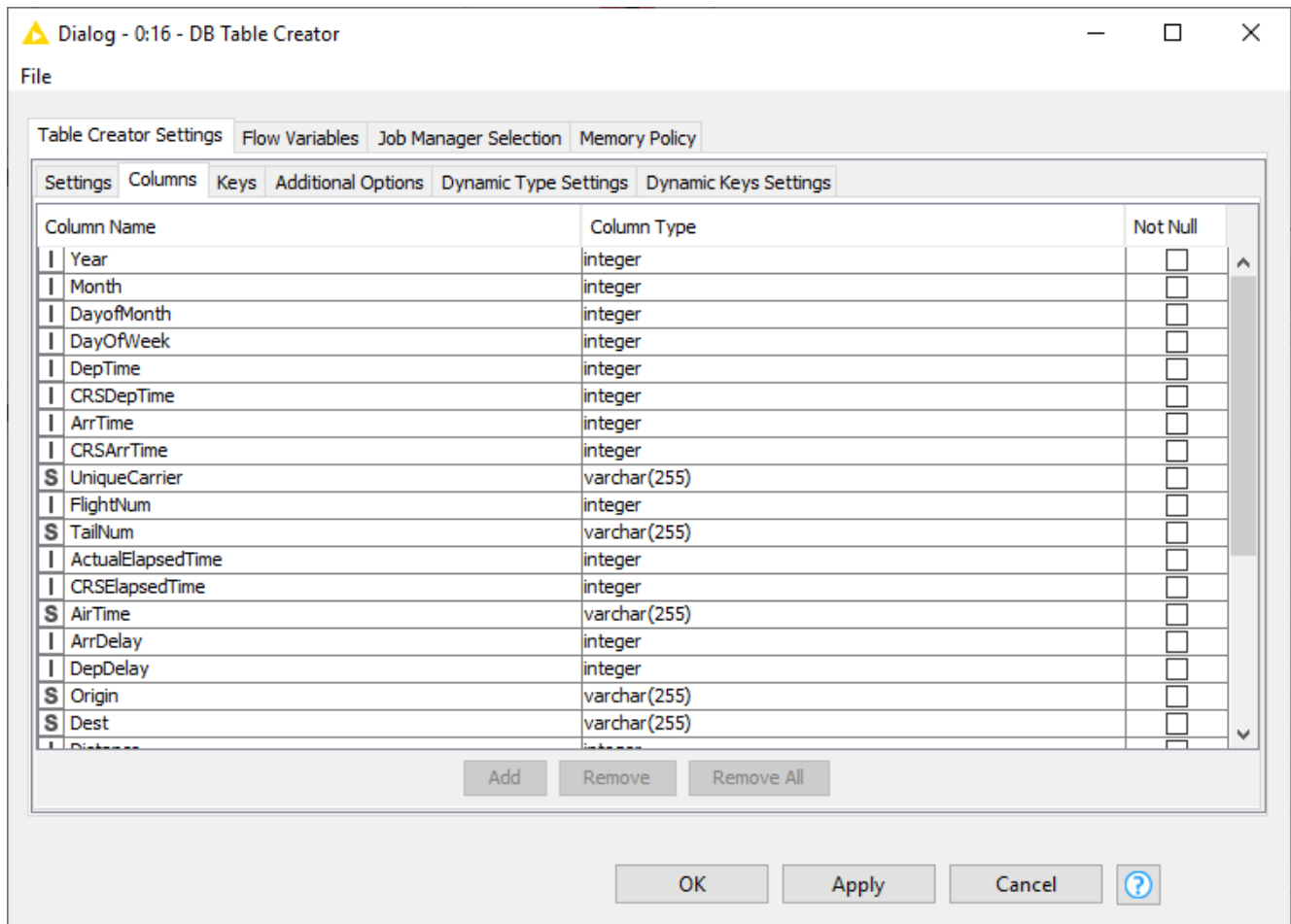
Figure 40. DB Table Creator: Columns
