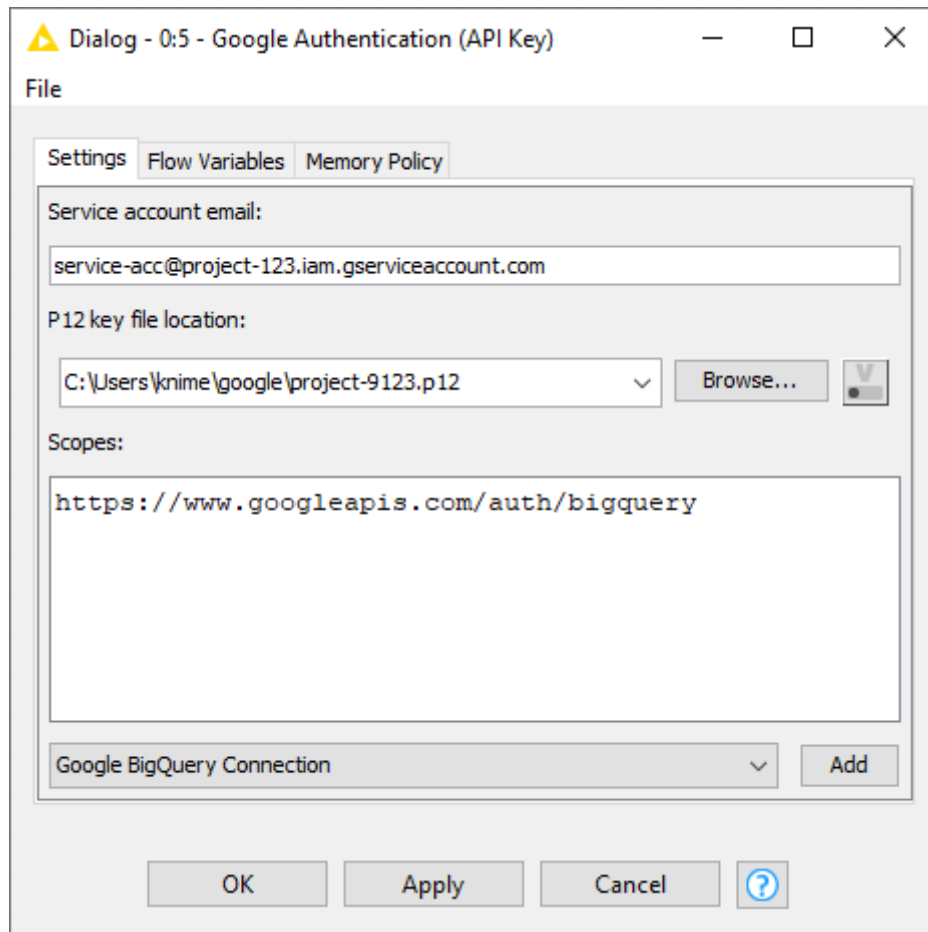
Figure 19. Configuration Window of Google Authentication (API Key) Node
