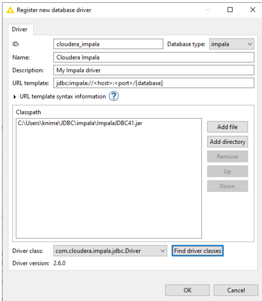
Figure 23. Register new Apache Impala driver
