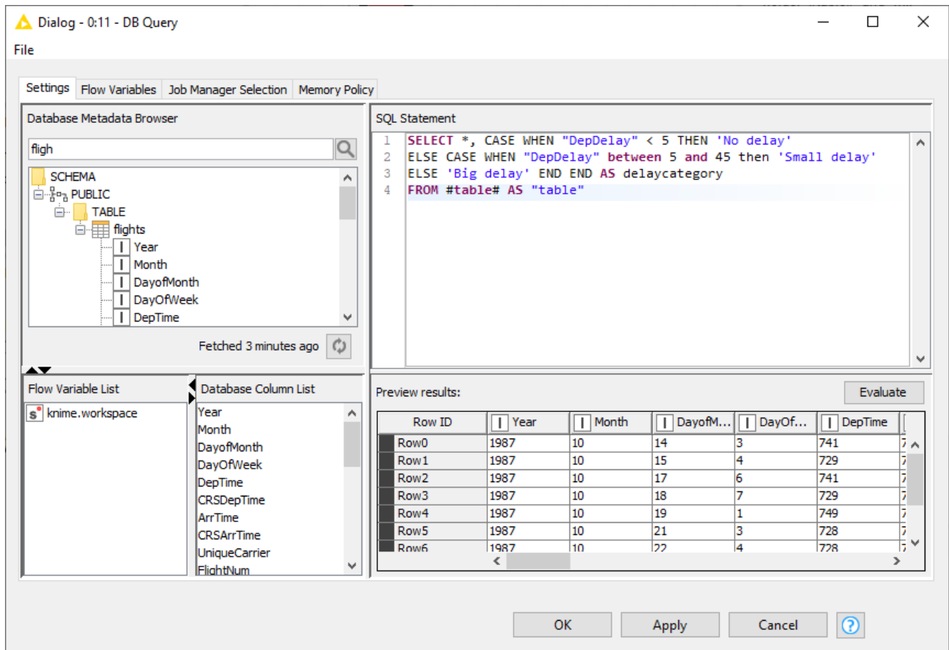
Figure 36. Configuration dialog of the DB Query node
